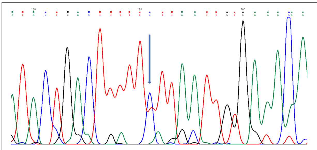
Figure 5. Chromatogram showing mutation of C>A at 4,947.0.
