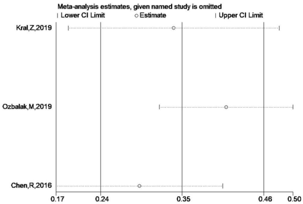
Supplementary Figure 1. Sensitivity analysis for OS.
